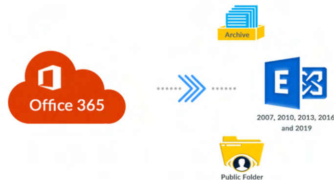
Offline 365 Migrations
